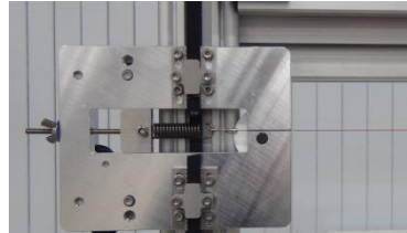
Tension system of the wire
